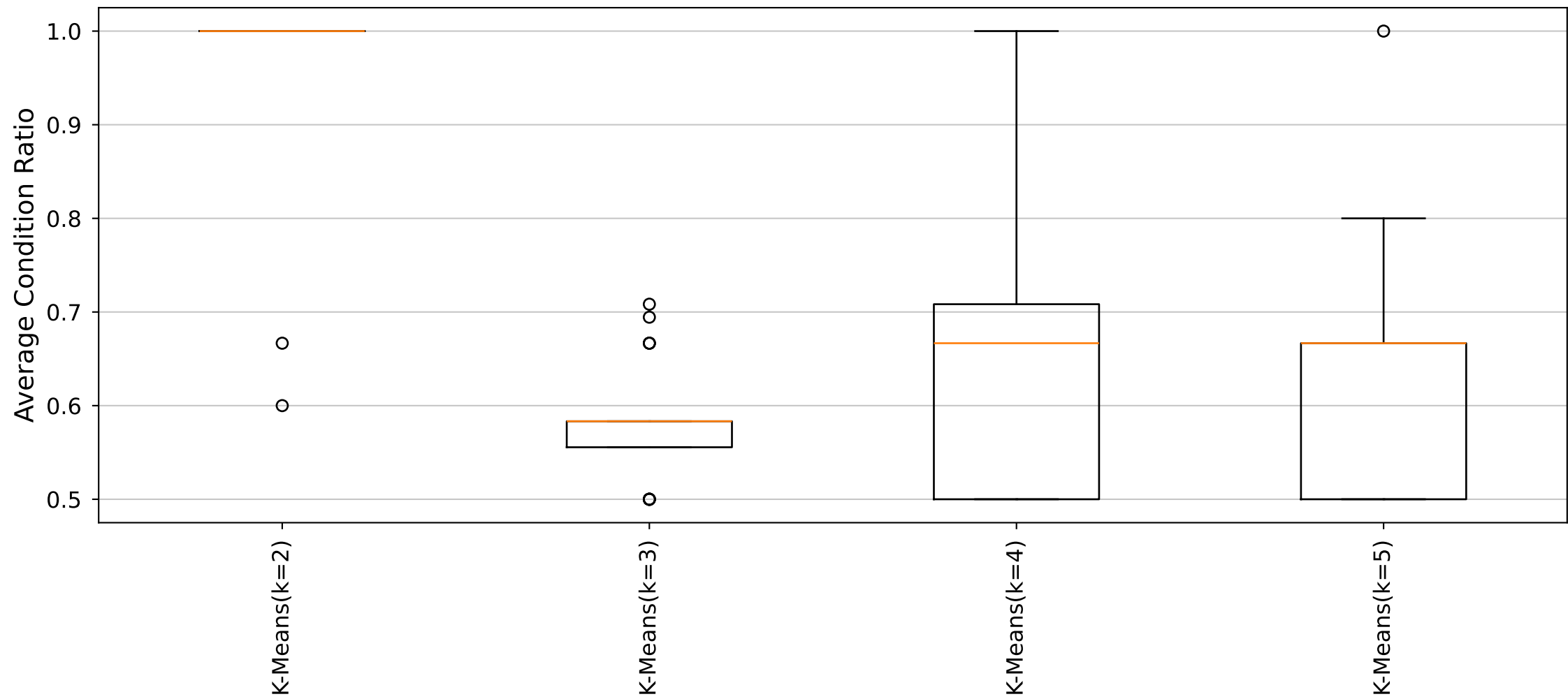
YARA Rules Average Condition Ratio Distribution (Cluster40_Size5 dataset)
